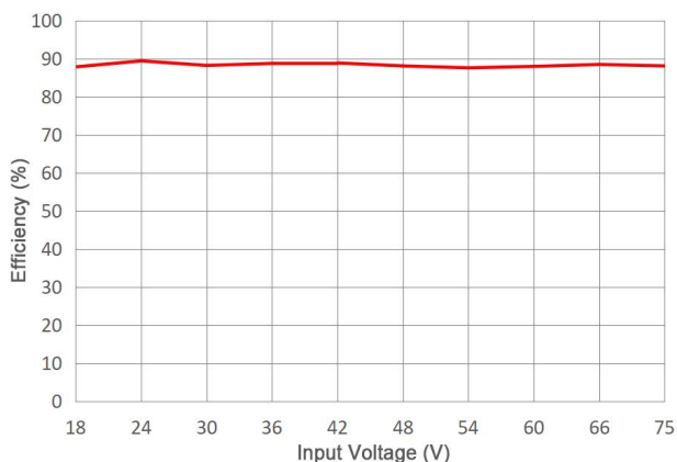
Efficiency VS Input Voltage (PFD6-36S12E2C3)
