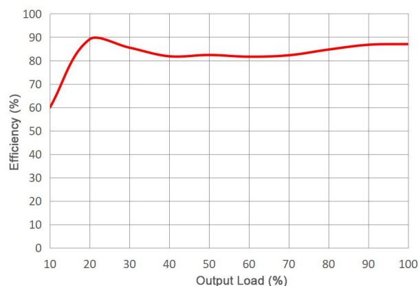
Efficiency VS Output Load (PFD6-18D15E2C3)
